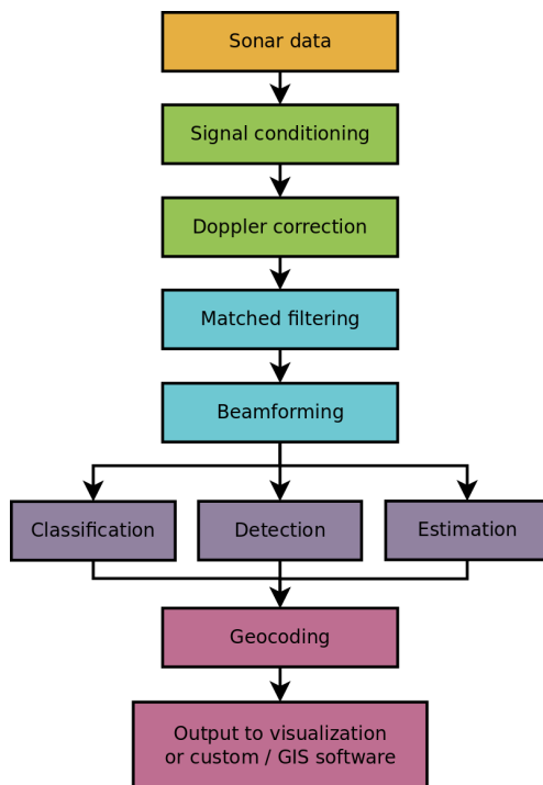
FIG. 22 Active sonar signal processing chain.
