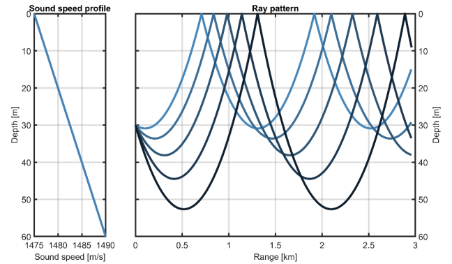
FIG. 7 Raytrace of sound in an upwards refracting environment.
