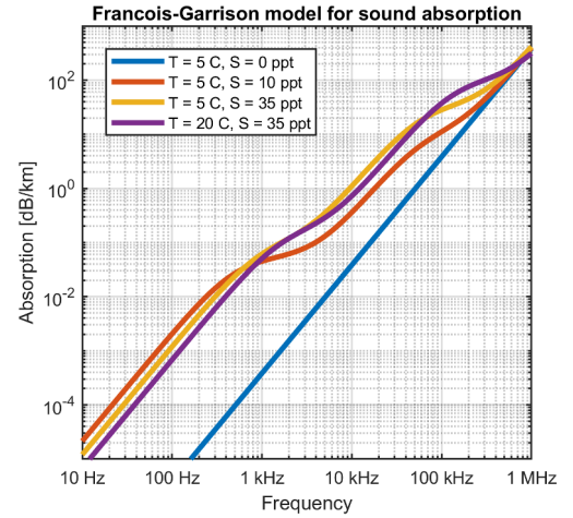
FIG. 4 Absorption coefficient in seawater.
