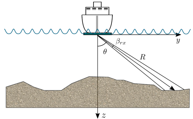
FIG. 26 Multibeam echosounder geometry.
