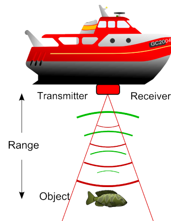
FIG. 23 Echosounding for fish finding.
