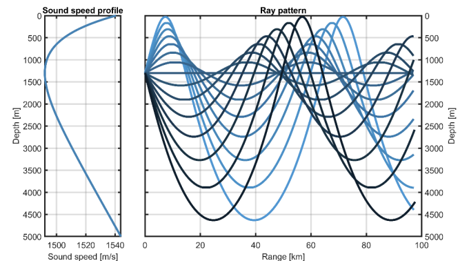
FIG. 8 Raytrace of sound in the deep water sound channel.
