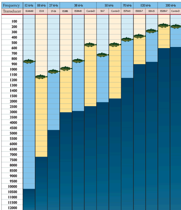
FIG. 24 Fish detection range (vertical axis) for different sonars operating at different frequencies. From www.simrad.com. Courtesy of Kongsberg Maritime.
