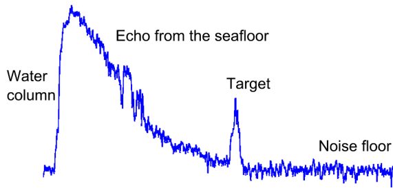
FIG. 21 Example range profile.
