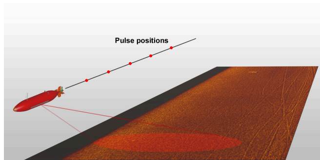
FIG. 31 Principle of synthetic aperture sonar.
