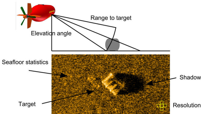
FIG. 33 Properties in a sonar image.
