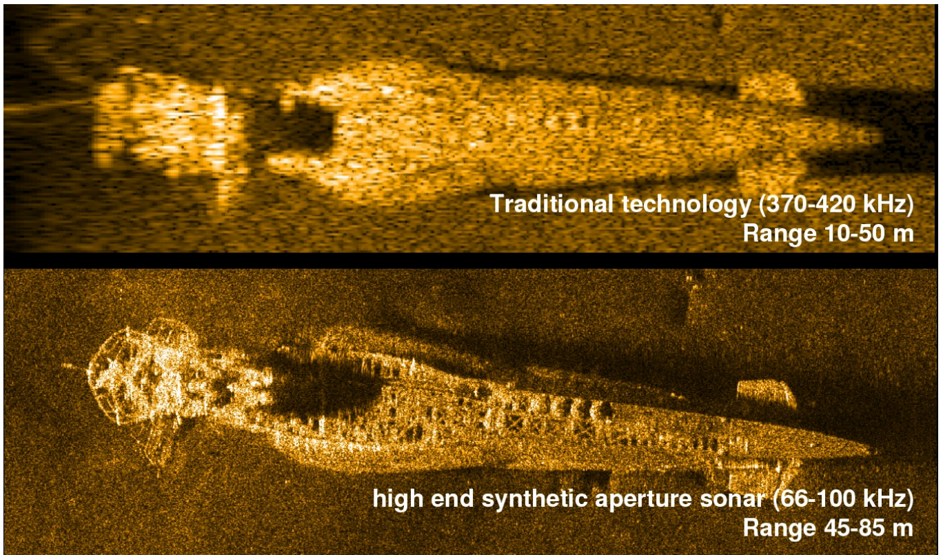
FIG. 34 Comparison of traditional sidescan sonar with synthetic aperture sonar. Images collected by HUGIN AUV. Courtesy of Kongsberg Maritime / FFL.
