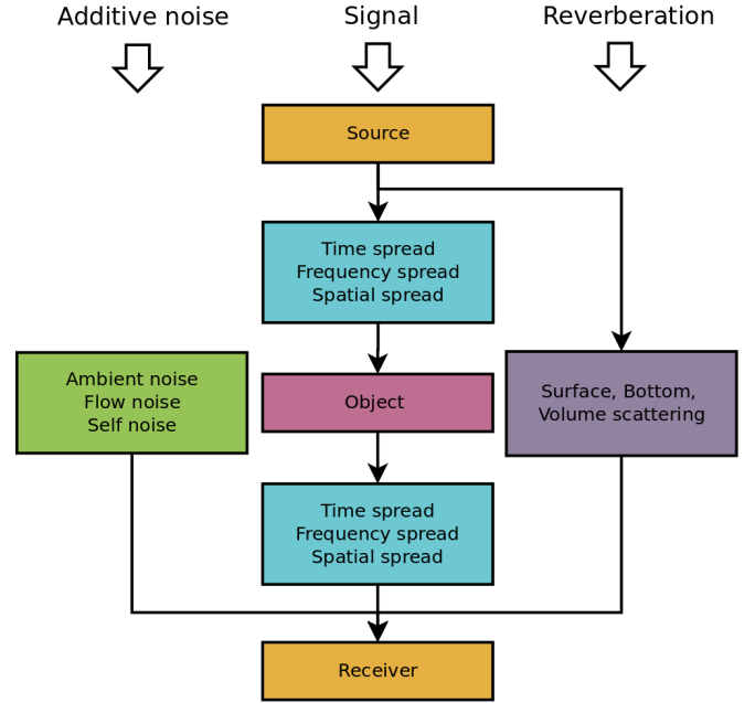
FIG. 20 Signal model.
