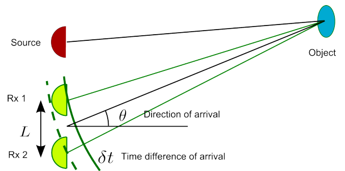
FIG. 17 Direction of arrival.
