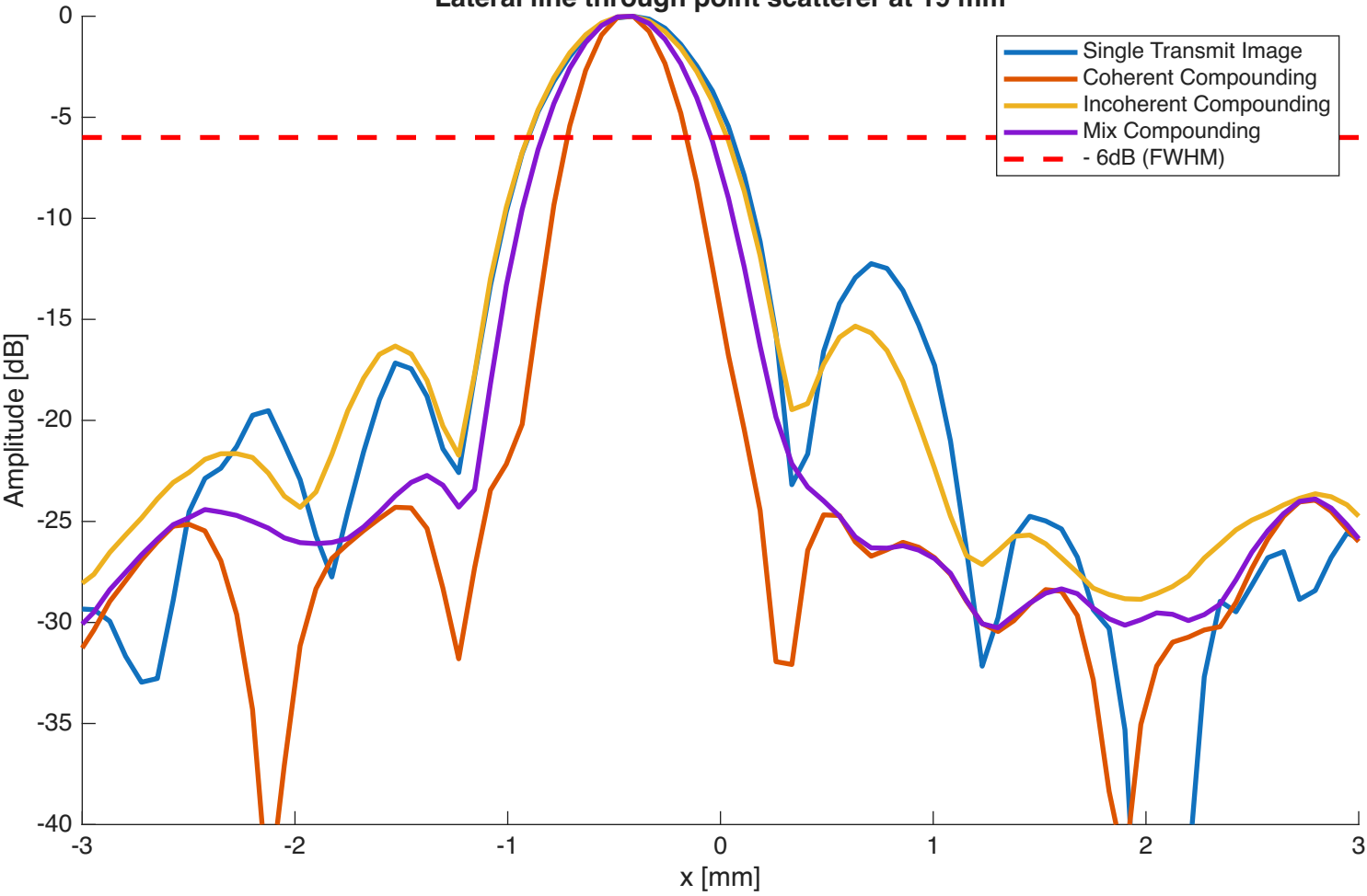
Lateral line through point scatterer at 19 mm
