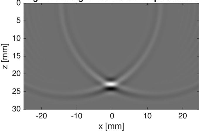
Image of the signal before envelope detection
