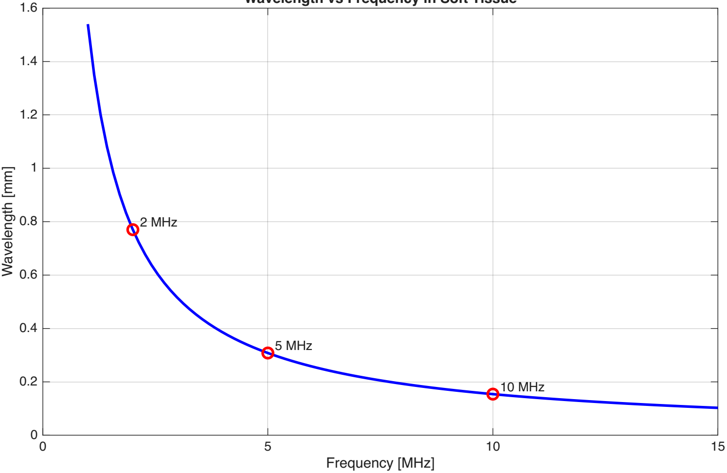
Wavelength vs Frequency in Soft Tissue
