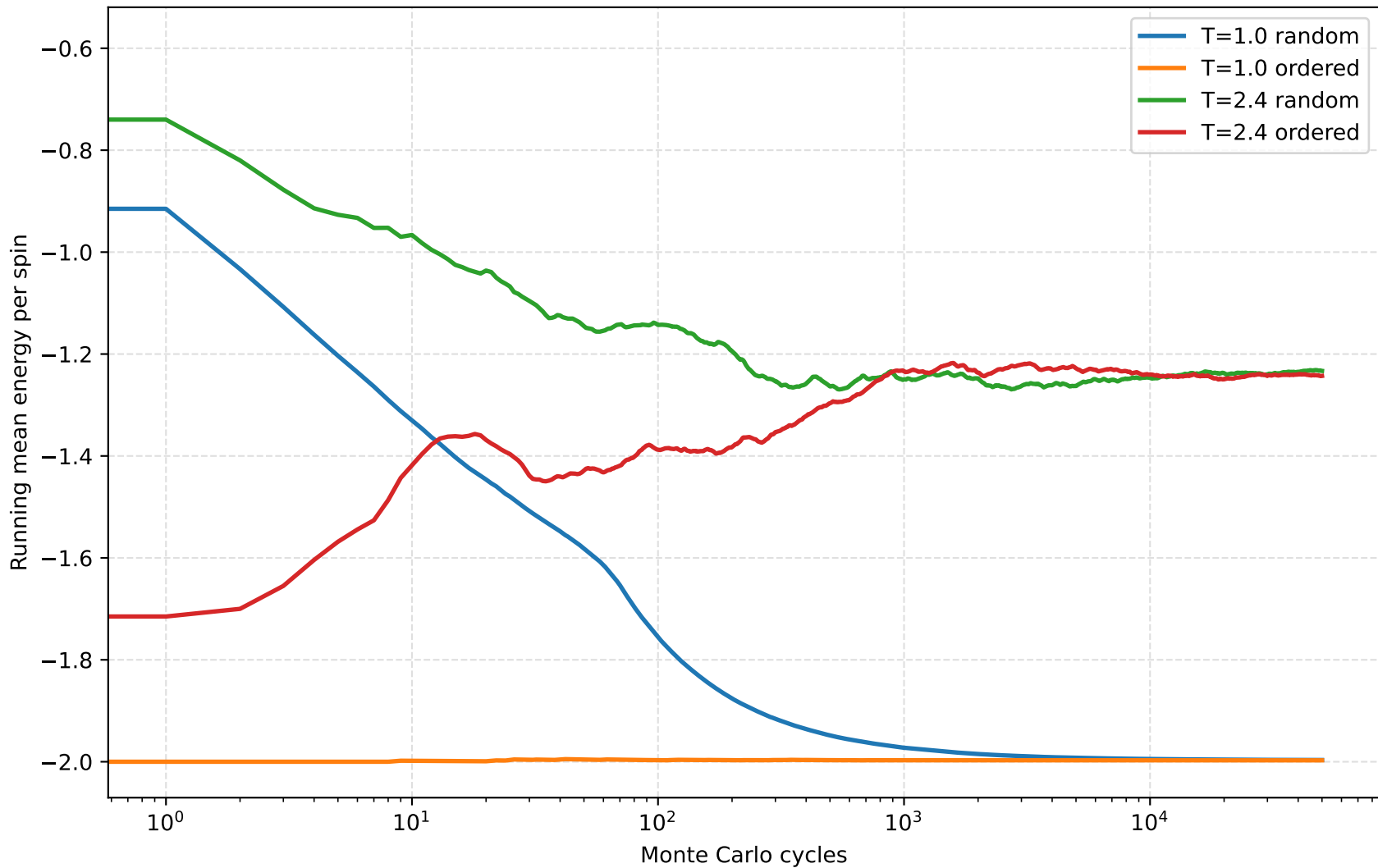
Running mean energy per spin vs Monte Carlo cycles
