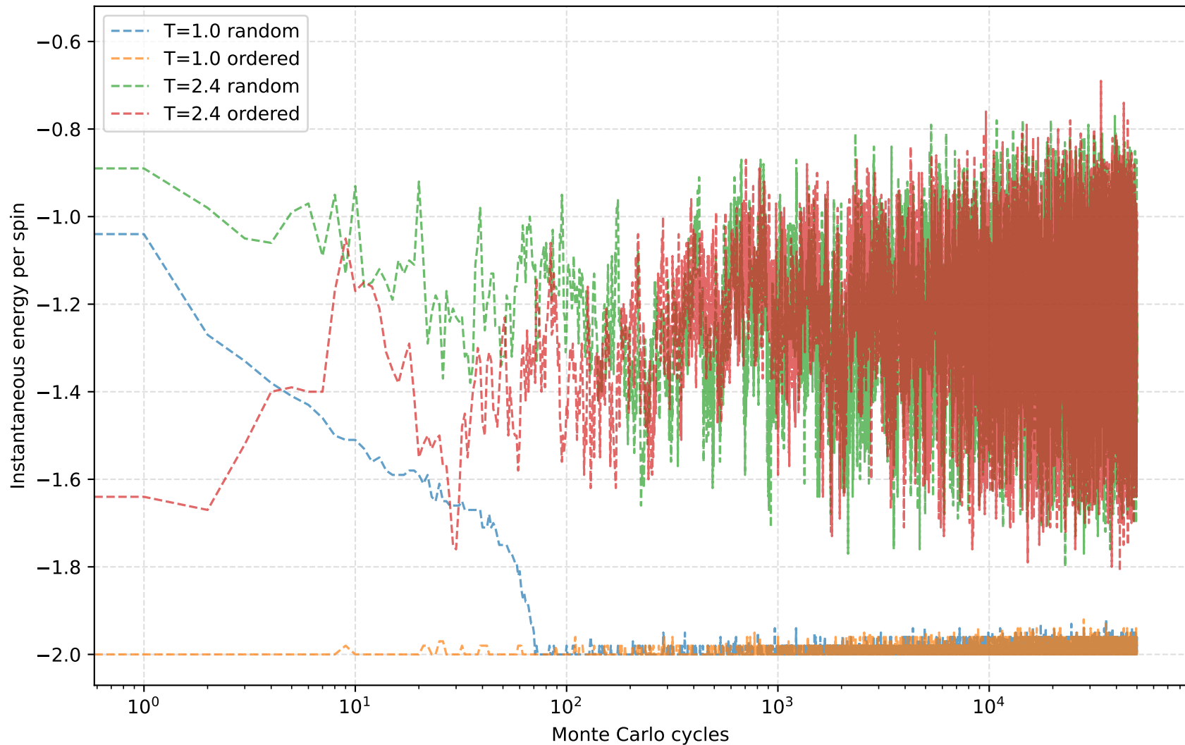
Instantaneous energy per spin vs Monte Carlo cycles
