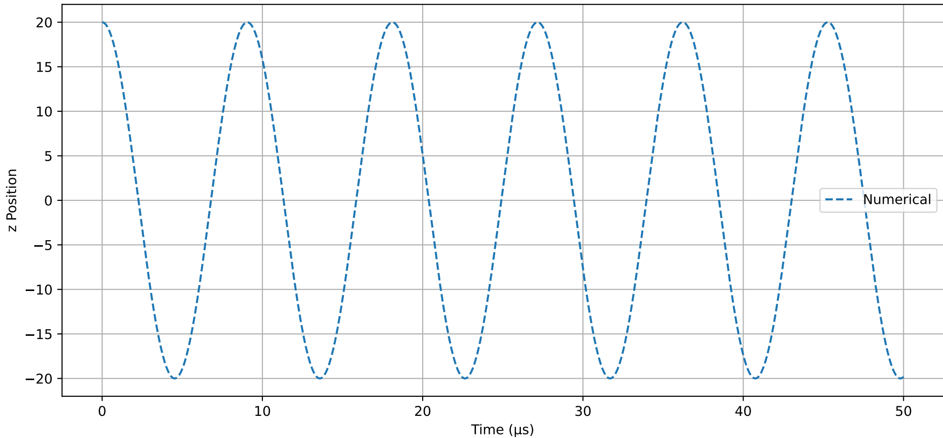
z-Motion: RK4 with n=8000
