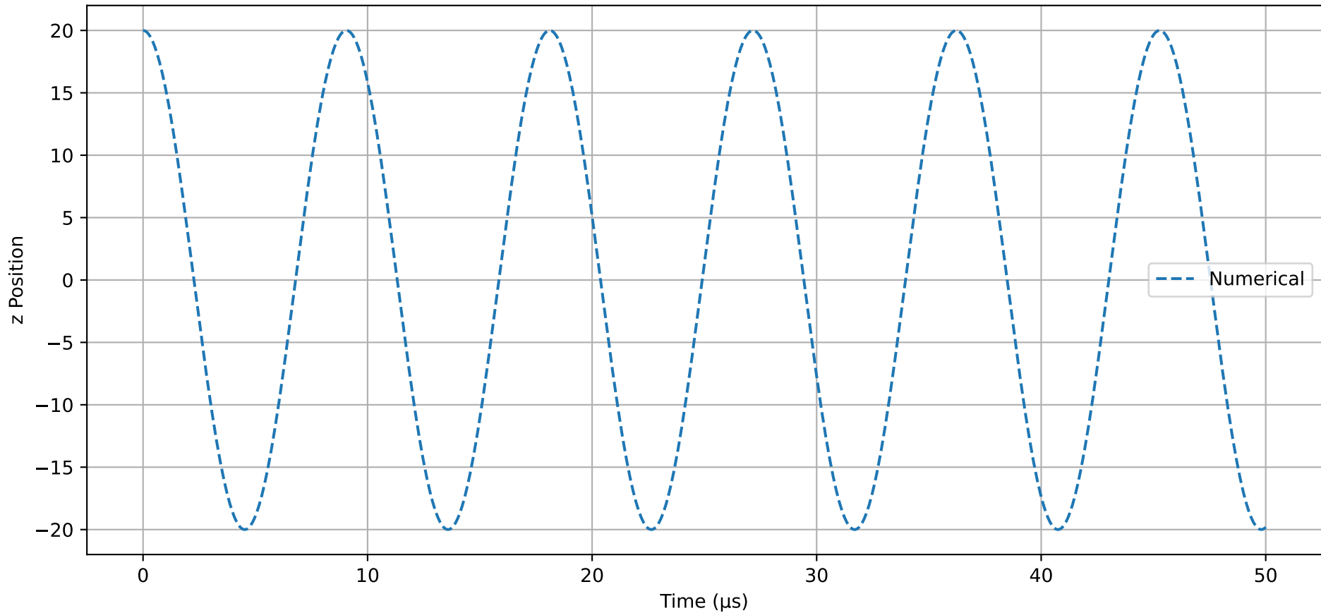
z-Motion: RK4 with n=4000
