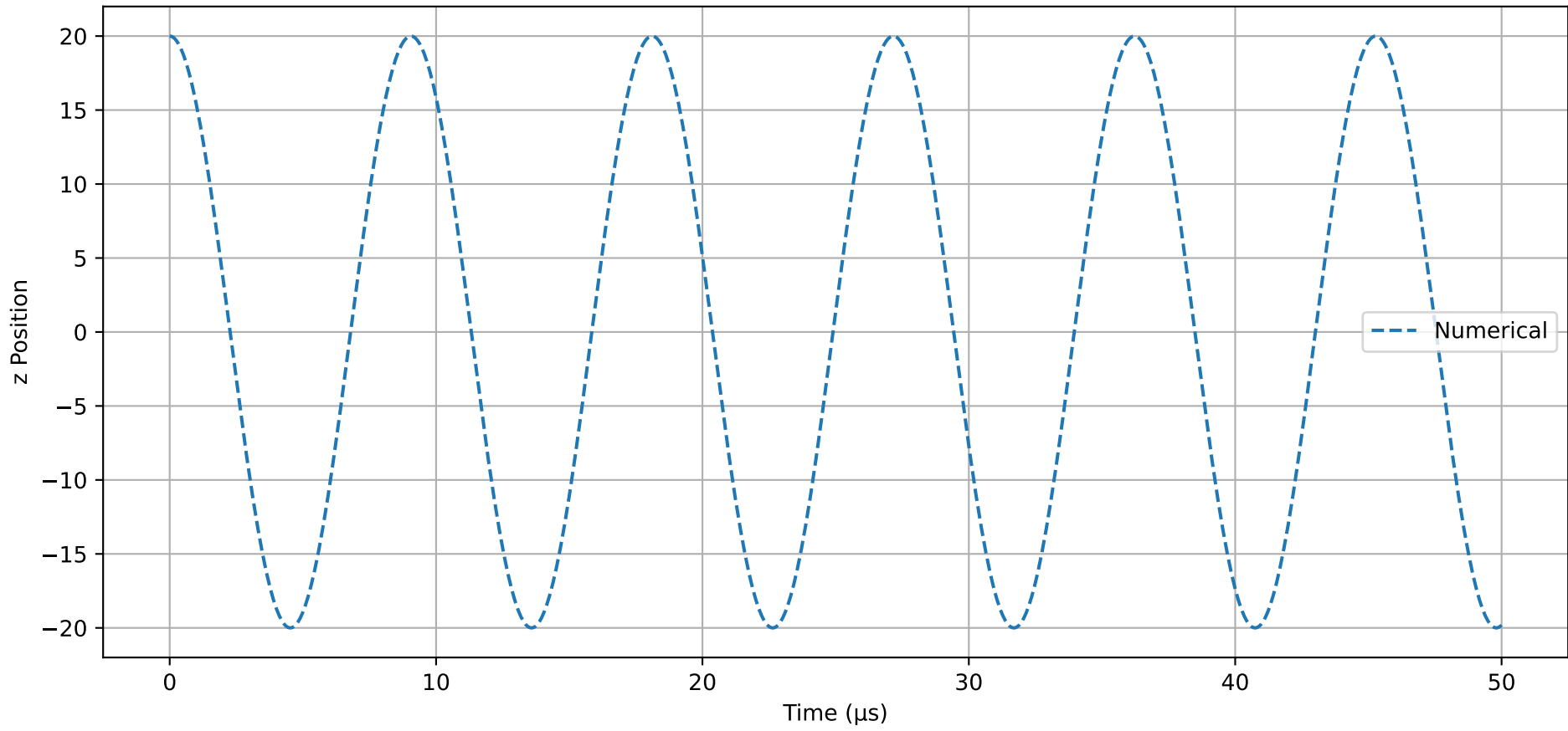
z-Motion: RK4 with n=16000
