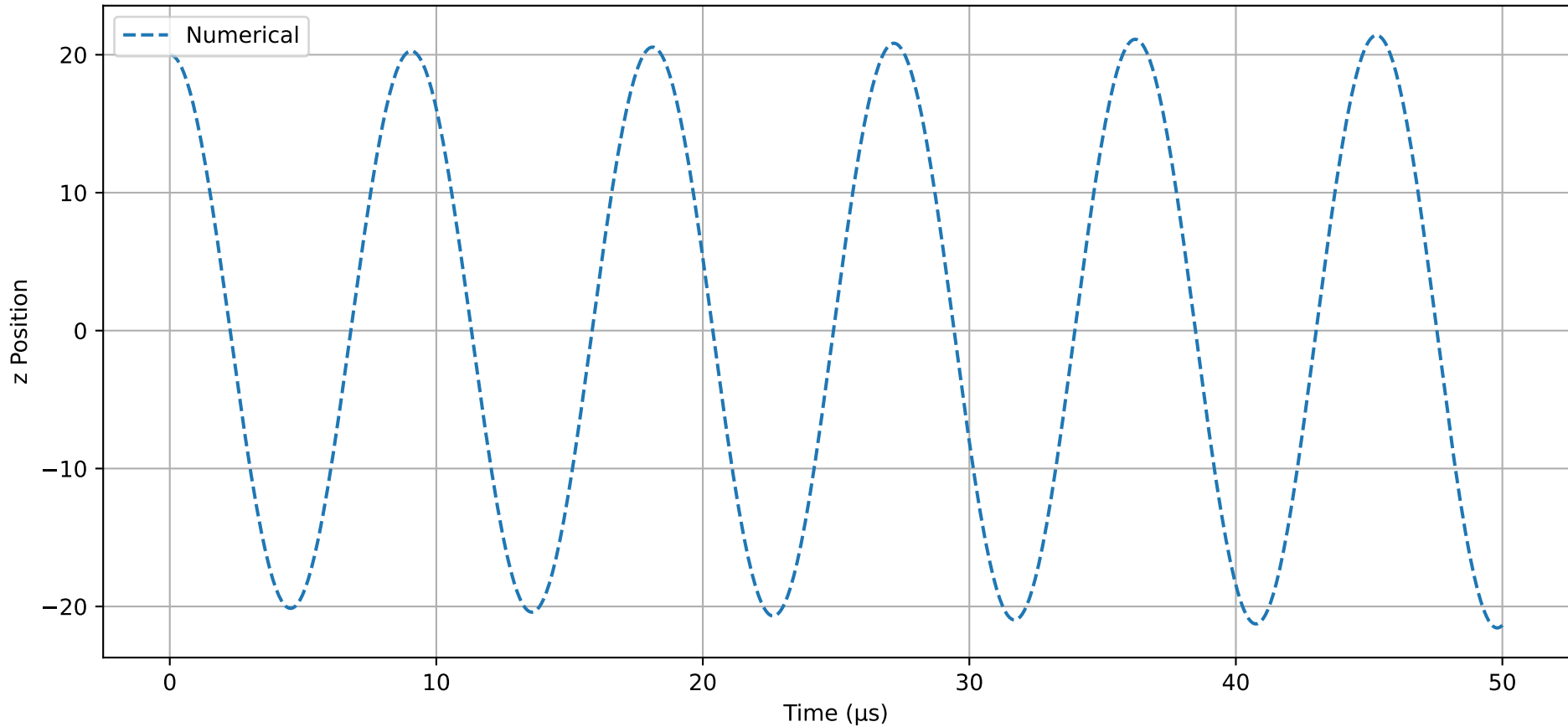
z-Motion: Euler with n=8000
