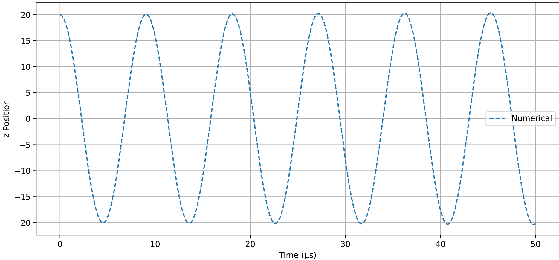
z-Motion: Euler with n=32000
