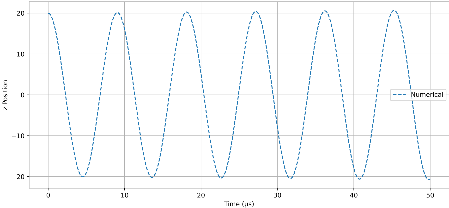
z-Motion: Euler with n=16000
