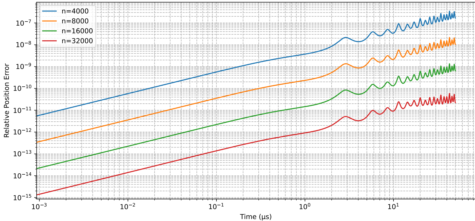
Relative Position Error vs Time (RK4)
