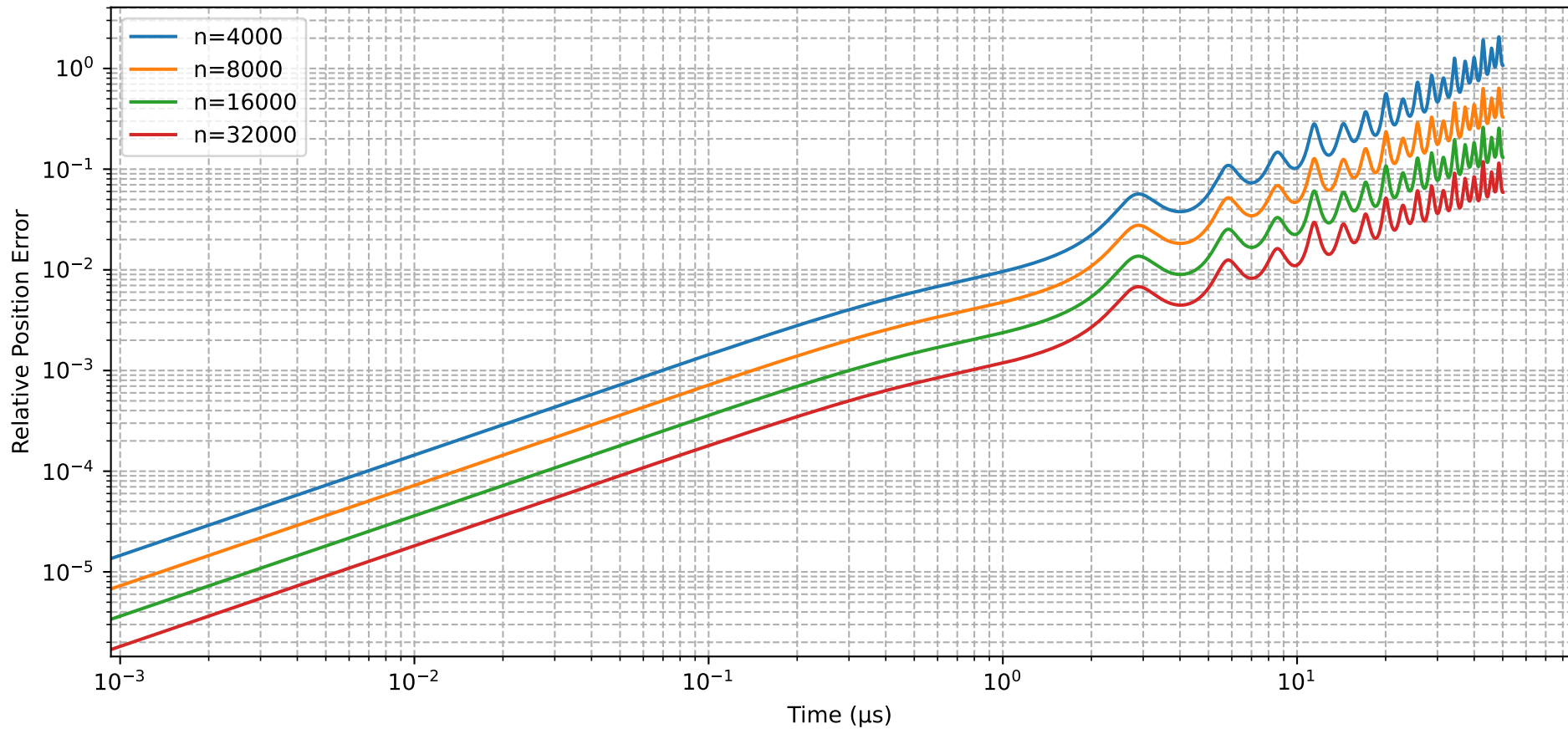
Relative Position Error vs Time (Euler)
