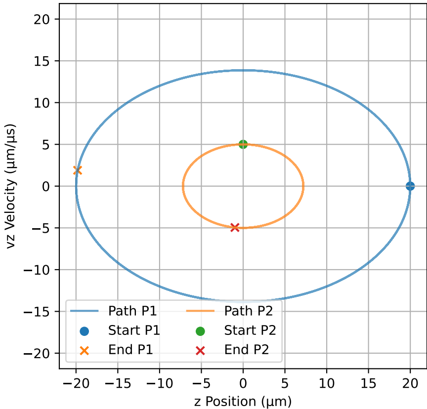
Z-vz Phase Space - No Interactions (T=50.0 \mu\text{s} )
