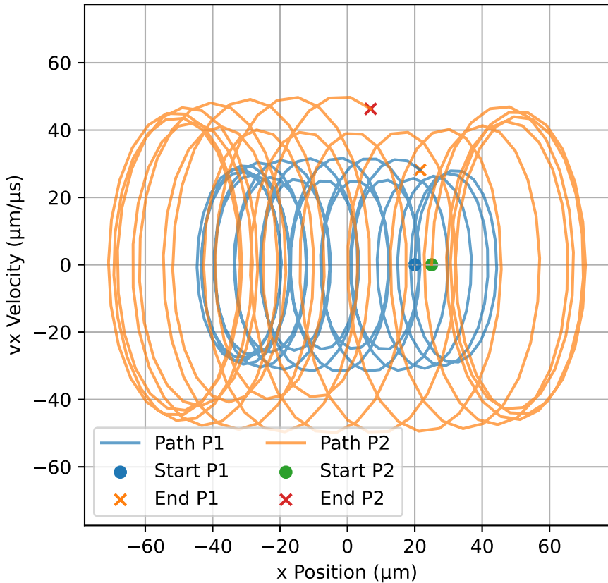
X- v_x Phase Space - No Interactions ( T=50.0 \mu\text{s} )
