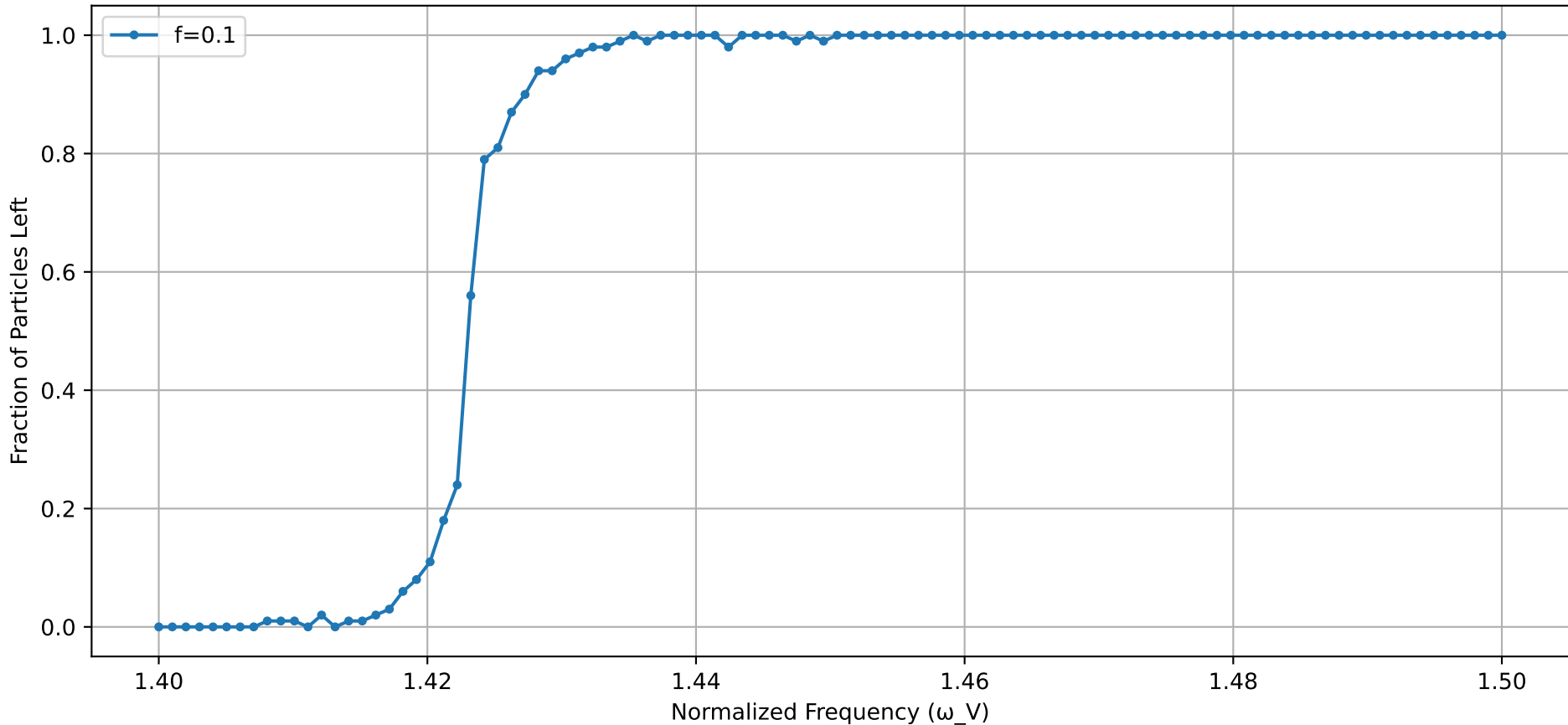
Particle Retention with Frequency: without Particle Interactions
