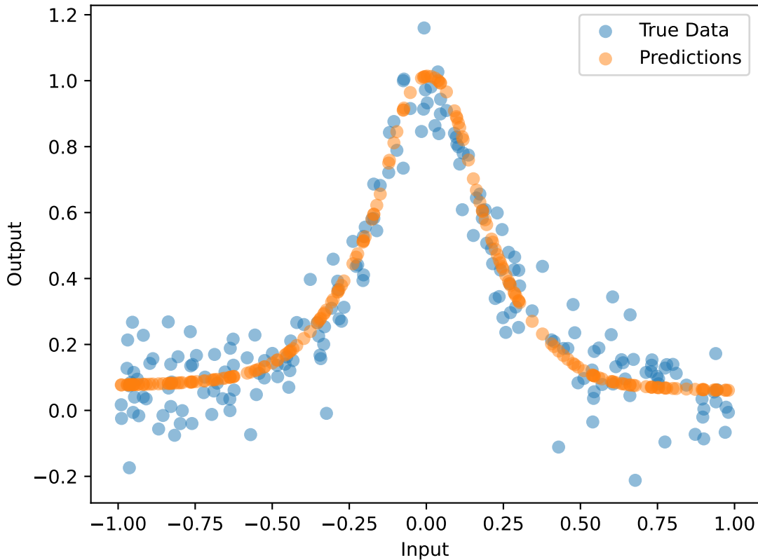
Neural Network Regression Predictions
